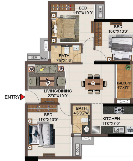
TYPICAL FLOOR 3RD TO 19TH
